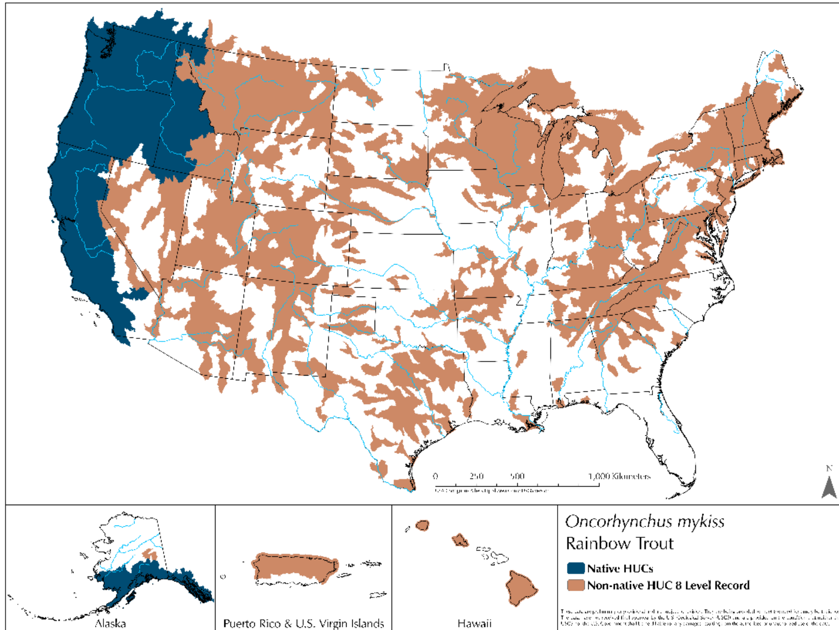
Figure 5-4. Native and non-native geographical distribution of rainbow trout/steelhead.
