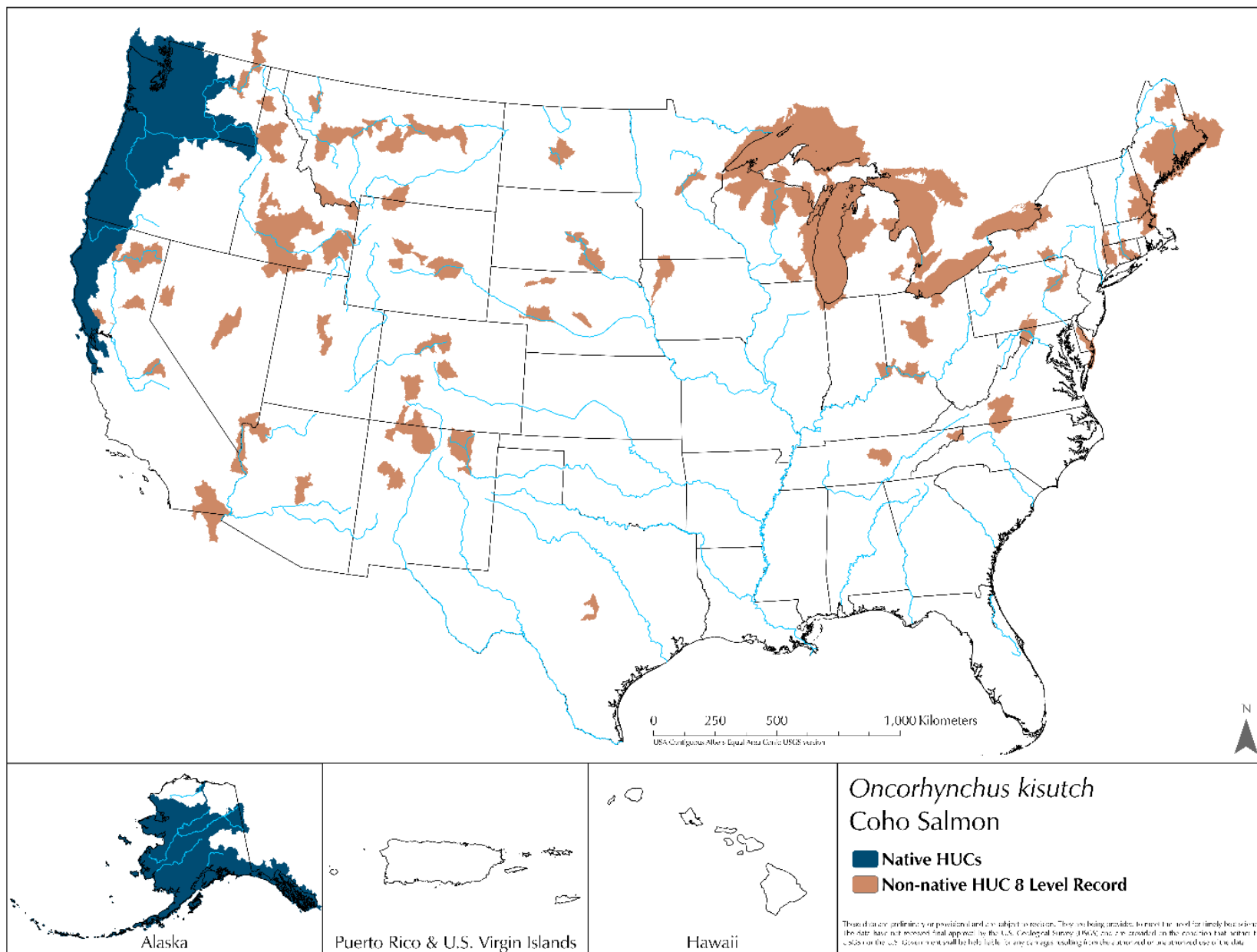
Figure 5-3. Native and non-native geographical distribution of coho salmon. Source: USGS Nonindigenous Aquatic Species (NAS) database.
